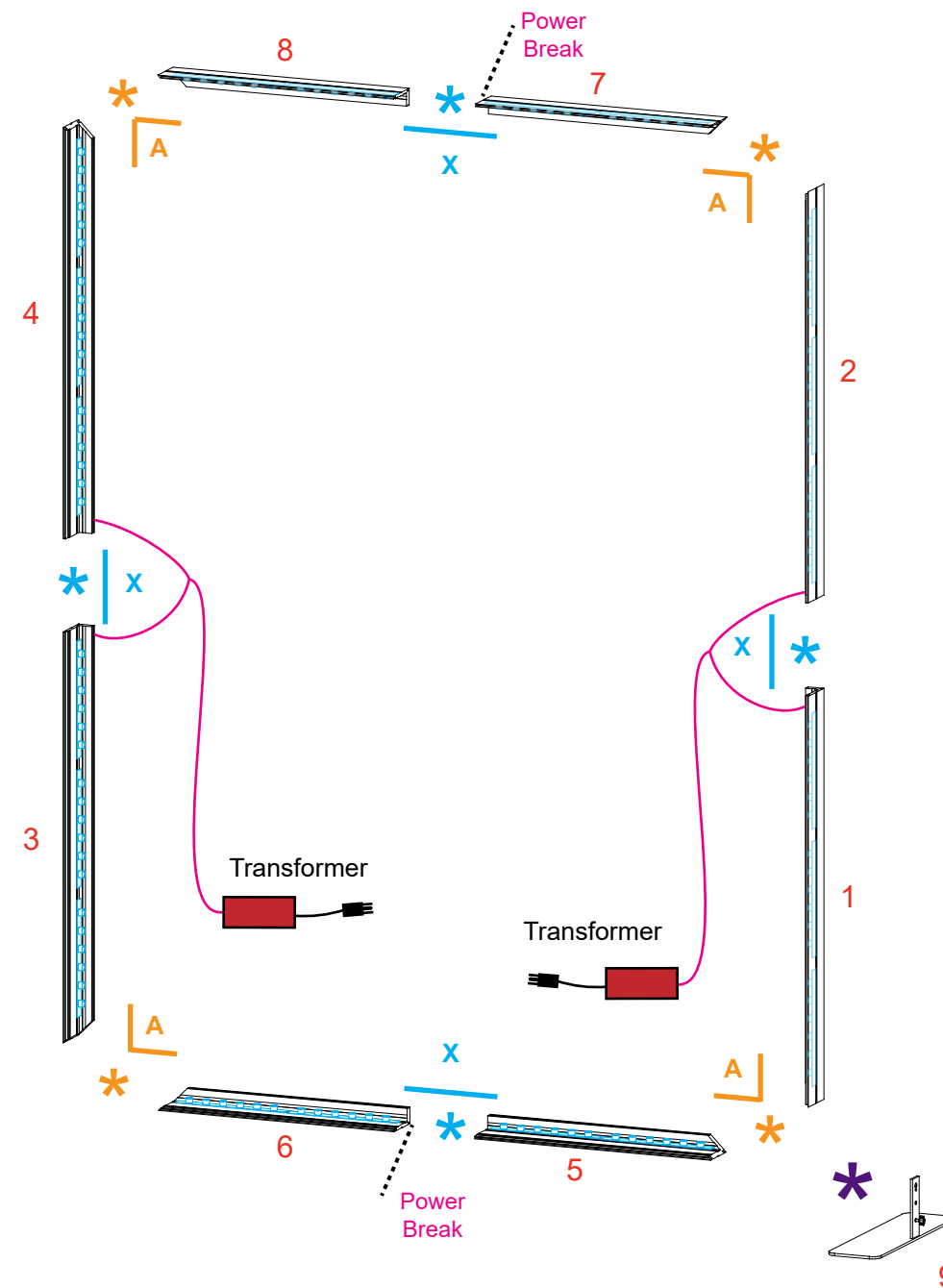
FRONT VIEW
